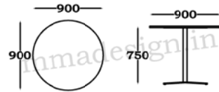
D 900 X H 750
