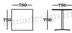
W 750 X D 750 X H 750
